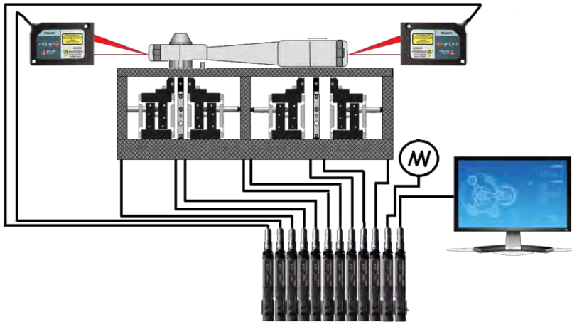
Solartron Flexure Contact Transducers and Non Contact Laser Triangulation Transducers. Connected to PC via USB Controller.
